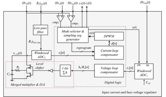
Fig. 9. Block diagram of the input current and bus voltage regulator.
