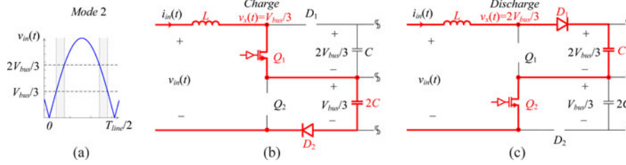
Fig. 4. Mode 2 of operation of the NSMB front-end stage: (a) input voltage range for mode 2; (b) equivalent circuit of the converter during inductor charging phase; and (c) equivalent circuit during the discharging.
