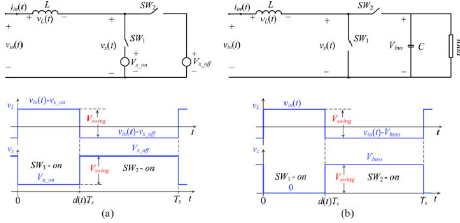
Fig. 2. Equivalent circuit for the analysis of the inductor voltage swing and the voltage waveforms of (a) a general boost-based converter and (b) the conventional boost.
