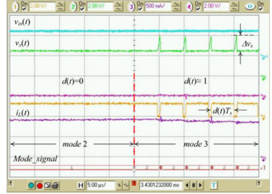
Fig. 21. Transitions from mode 1 to mode 2 (top) and from mode 2 to mode 3 (bottom); Ch. 1 (top): input line voltage, v_{in}(t) (200 V/div); Ch. 2 (upper middle): switching node voltage, v_x(t) (200 V/div); Ch. 4 (middle): gating signal of SW_1 , c_1(t) (20 V/div); Ch. 1 (lower middle): gating signal of SW_2 , c_2(t) (20 V/div); Ch. 3 (bottom): input line current, i_L(t) (0.5 A/div); digital input: mode control signal ((0 = mode 1, 1 = mode 2, 2 = mode 3). Timescale is 5 \mu s/div. Operating conditions v_{line} = 220 V rms , V_{bus} = 400 V, P_{out} = 100 W, C_{top} = 150 mF, C_{bottom} = 300 mF, L = 230 mH.
